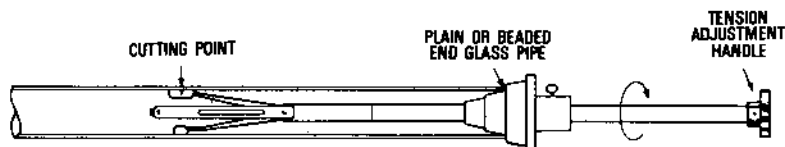
Complete Cutter
